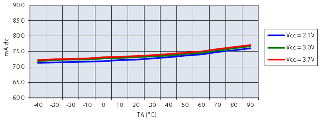
Current consumption in TX vs. temperature (CW mode)
